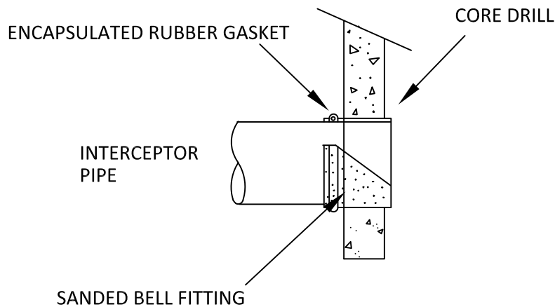
SAND COLLAR
