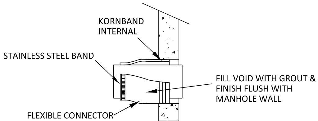
FLEXIBLE CONNECTOR
