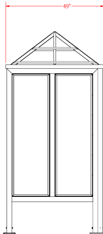
SIDE VIEW SCALE: 1/16"=1"
